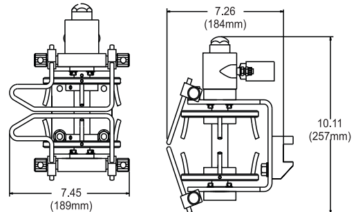
582xx586 TR500M Pneumatic tab trim removal system, 30psi maximum
