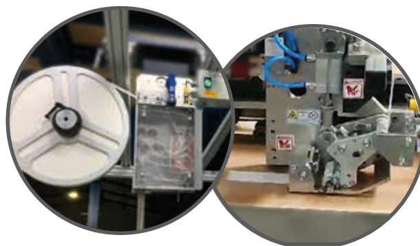
Release liner accumulator and release liner tape applicator
