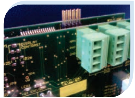
Photo-eye Connections
